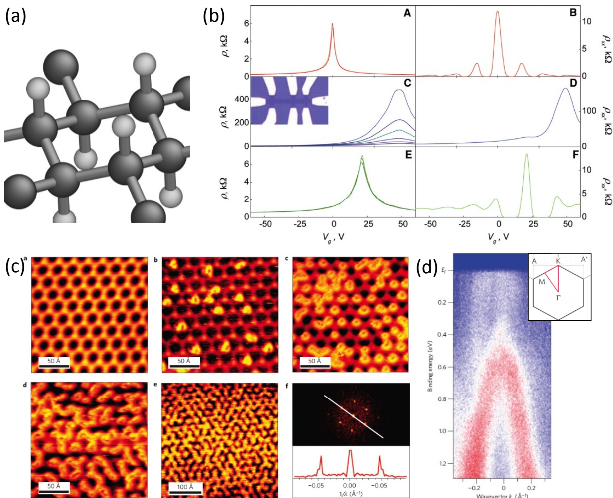
Figure 4. (a) The structure of graphene with chair conformation, which can be viewed as fused cyclohexane. (b) Measured resistivity without magnetic field ( \rho ) at different temperatures and with magnetic field ( \rho_{xx} ), before hydrogenation (A and B), after hydrogenation (C and D), and after hydrogen desorption (E and F). 79 Inset, the micrograph of the typical Hall measurement setup. (c) STM micrographs of graphene with various degrees of hydrogenation (a-e), where hydrogen atoms are the bright spots or areas. Panel f is the Fourier transform of the micrograph in panel e. 85 (d) Angle-resolved photo emission intensity of hydrogenated graphene along A-K-A' (see inset). 85 (Reprinted with permission from ref. 79 , Copyright© 2009 AAAS; ref. 85 , Copyright© 2010 Macmillan Publishers Ltd: Nature Materials.)
