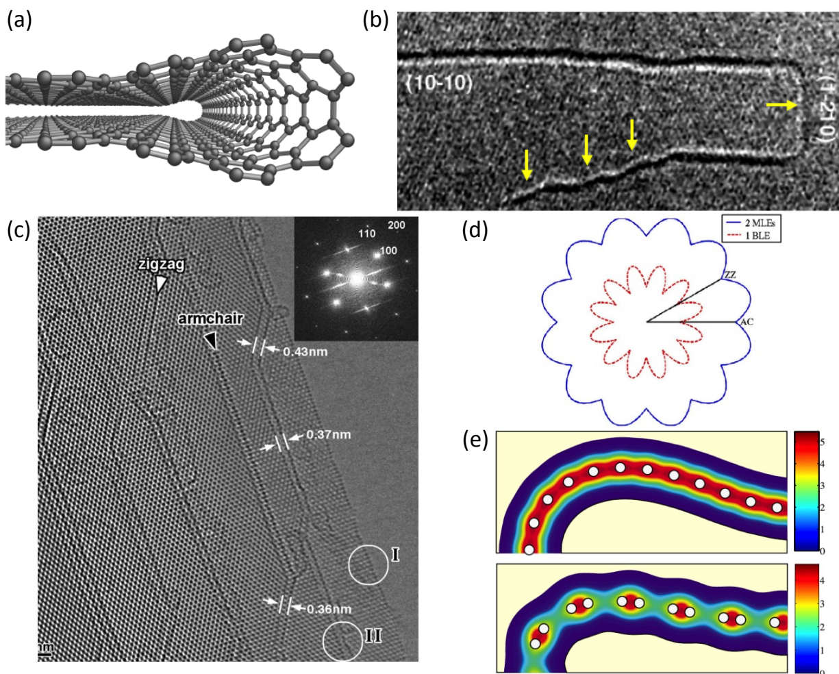
Figure 6. (a) The atomic structure of a zigzag bilayer edge termination. (b) Transmission electron microscopic (TEM) micrograph of BLEs formed from Joule heated sublimation process. 8 Both zigzag and armchair inclinations are observed. (c) TEM micrograph with atomic resolution of multiple BLEs formed from annealing graphite powder at 2000 °C for 3 hours. 123 (d) Semi-quantitative Wulff plots for mono- and bilayer edge terminations in polar representation. 124 (e) Computed (density functional theory) valence electron density of armchair (top) and zigzag (bottom) BLEs, demonstrating the Coulombic relaxation of electron density from inside of the BLE to the outer surface. 130 (Reprinted with permission from ref. 123 , Copyright© 2009 American Physical Society.)
