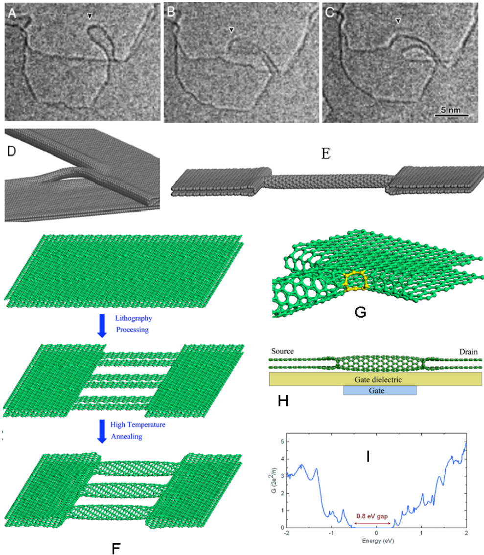
Figure 7. Carbon nanostructures formed in situ on graphene substrate by Joule-heating. A-C shows two neighboring bilayer graphene interconnected by a carbon nanotube, as pointed out by the arrowheads. D, E, F and G are atomic structural models. Panel F shows one possible patterning process, supported by MD simulation. 122 In G we can see a nine-sided polygon, highlighted by yellow color, amidst the hexagonal bonding network of graphene, which is a geometrically disinclination at the interface between flat and curved carbon. H shows a FET device model (side view) based on single-wall carbon nanotube and bilayer graphene hybrids. Panel I shows the calculated electronic conductance spectrum of the metal-semiconductor-metal (flat graphene-nanotube-flat graphene) junction device, 122 where the intrinsic transport gap of the nanotube is preserved.
