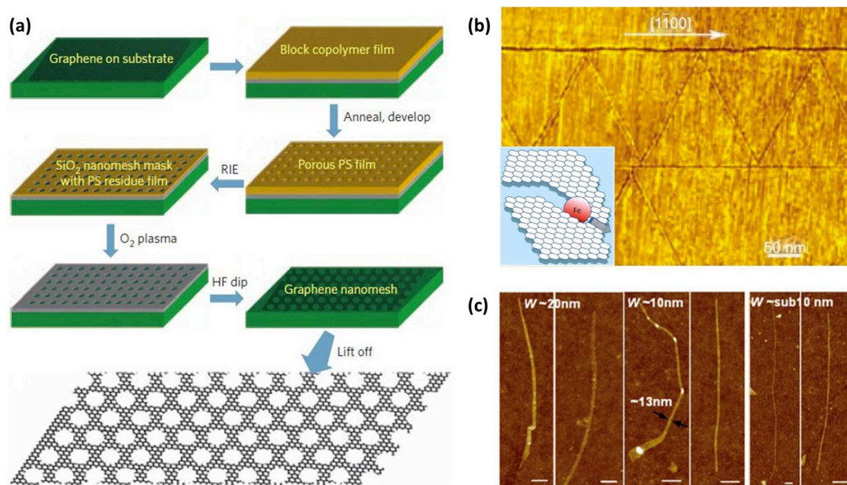
Figure 2 (a) Schematic of fabricating graphene nanomesh by block copolymer lithography. Block copolymer thin film with periodic cylindrical domains was first formed and annealed on top of SiO x -protected graphene flake to develop porous polymer film. Fluoride-based reactive ion etching and oxygen plasma etching were then used to punch holes into the graphene layer and remove the polymer film. Finally graphene nanomesh was obtained by dipping the sample into HF solution to remove the oxide mask. 48 (b) Atomic force micrograph of triangular flakes from cutting graphene by catalytic methanation. 51, 52 The scale bar measures 50 nm. Inset: a schematic of the etching process by a migrating catalytic metal nanoparticle. (c) Atomic force micrographs of slender GNRs from mechanochemical approach. 4 Bars all correspond to 100 nm. (Reprinted with permission from ref. 48 , Copyright© 2010 Macmillan Publishers Ltd: Nature Nanotechnology; ref. 51 , Copyright© 2008 American Chemical Society; ref. 52 , Copyright© 2008 Springer; ref. 4 , Copyright© 2008 AAAS.)
