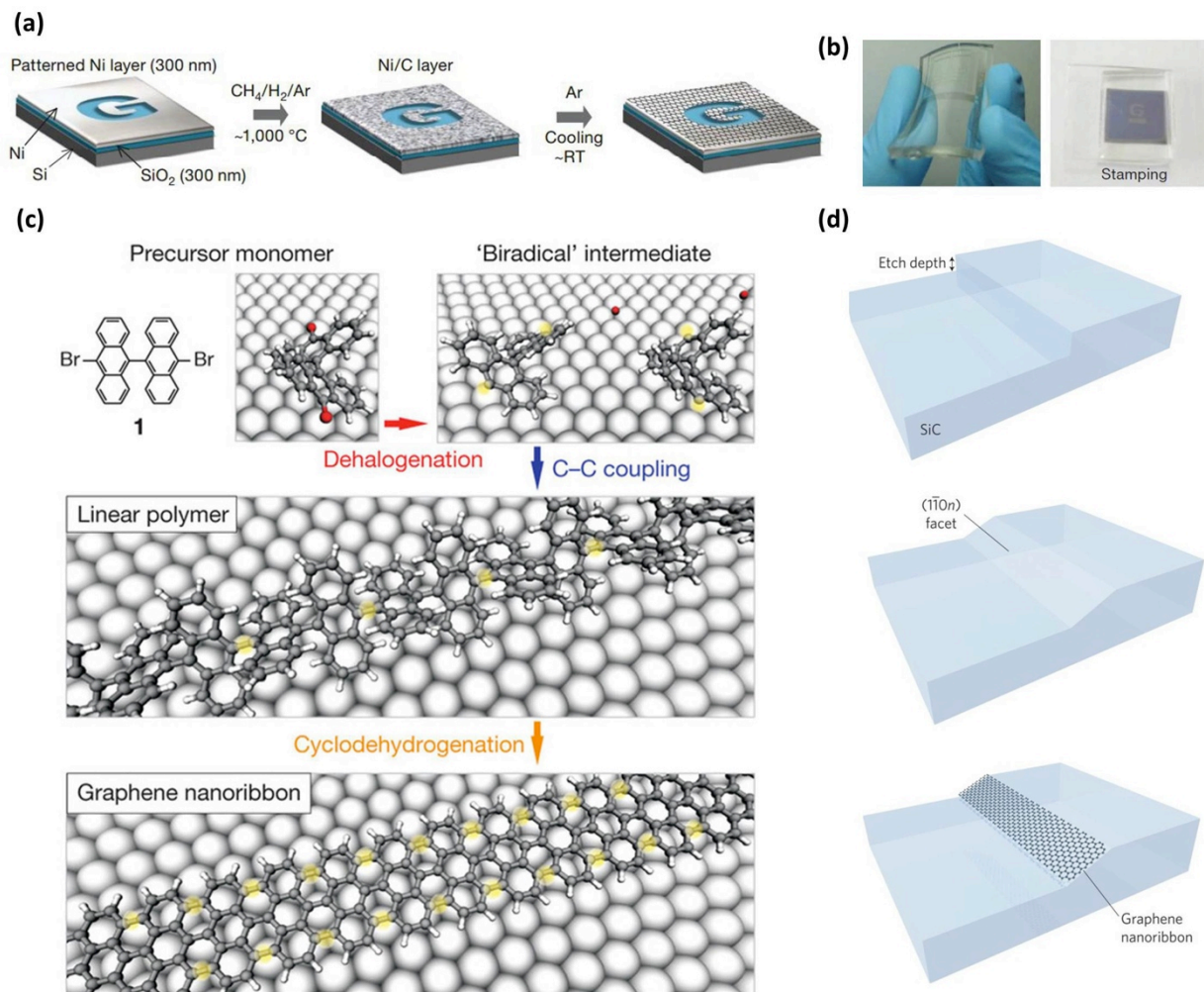
Figure 3 (a) Schematic of patterned growth of graphene on a pre-patterned catalytic surface, and (b) the resultant flexible graphene on a transparent elastomeric substrate, and the patterned graphene transferred onto a SiO 2 substrate. 59 (c) Schematic of bottom-up fabrication of atomically precise GNRs. Top, precursor monomers were first deposited onto clean metal substrates using thermal sublimation. Dehalogenation was also induced during this step. Middle, formation of linear polymers by covalent interlinking of the dehalogenated intermediates. Bottom, Annealing at higher temperature introduces intramolecular cyclodehydrogenation and leads to hydrogen-terminated fully aromatic GNR. 61 (d) Self-organized graphene nanoribbon formation on SiC. A nanometre-scale step is etched into SiC crystal by fluorine-based reactive ion etching. The crystal is then heated to 1200-1300 °C, which induces step flow and relaxation to the (11̄0n) facet. Upon further heating to ~1450 °C, self-organized graphene nanoribbon forms on the facet. 63 (Reprinted with permission from ref. 59 , Copyright© 2009 Macmillan Publishers Ltd: Nature; ref. 61 , Copyright© 2010 Macmillan Publishers Ltd: Nature Nanotechnology; ref. 63 , Copyright© 2010 Macmillan Publishers Ltd: Nature Nanotechnology.)
