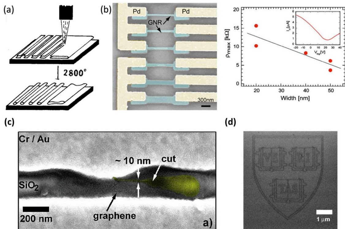
Figure 1 (a) A visionary insight into graphene carving long before the isolation of graphene. 33 . The schematic proposed by Ebbesen and Hiura involves mechanically cutting graphene bilayers with scanning probes, followed by subsequent annealing, to fabricate pre-designed carbon nanostructures. (b) Graphene nanoribbons with controlled widths fabricated by e-beam lithography, and the measured electric resistivity of GNRs as a function of their widths. 39 (c) A suspended graphene device after etching with helium ion lithography. Minimum feature size about 10 nm can be achieved. 43 (d) The same authors also demonstrated that complex patterns can be created on multi-layer graphene flake using this technique. 44 (Reprinted with permission from ref. 33 , Copyright© 1995 WILEY-VCH; ref. 39 , Copyright© 2007 Elsevier; ref. 43 , Copyright© 2009 American Chemical Society; ref. 44 , Copyright© 2009 IOP Science.)
